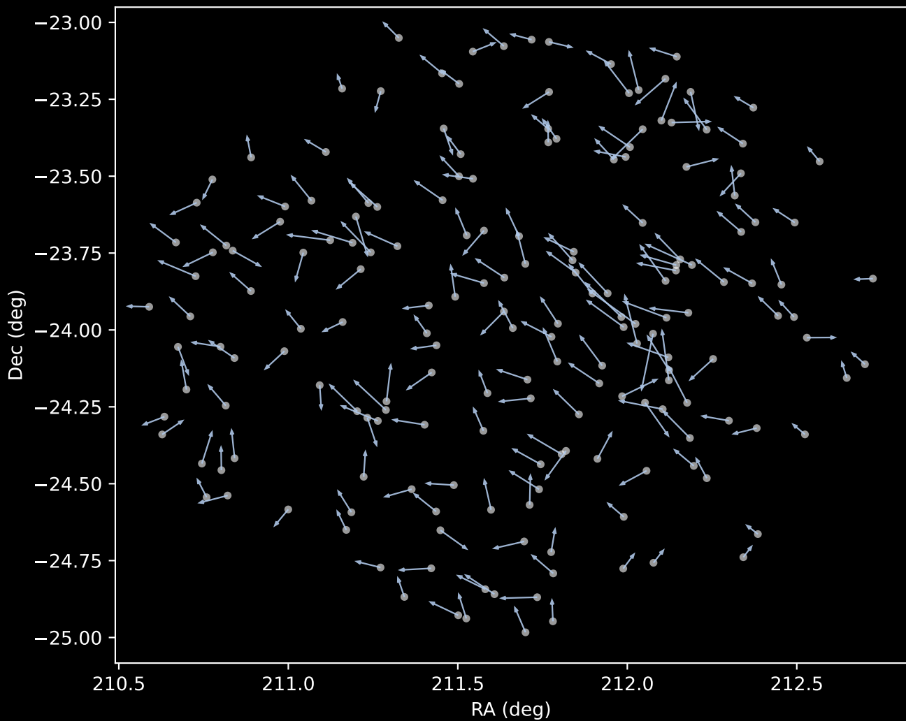
GALAH DR4 Cluster 1 Proper Motion Vectors (n=184)
