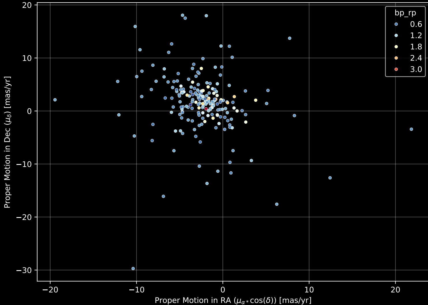
GALAH DR4 Field: [8439] Proper Motion Diagram (n= 206)
