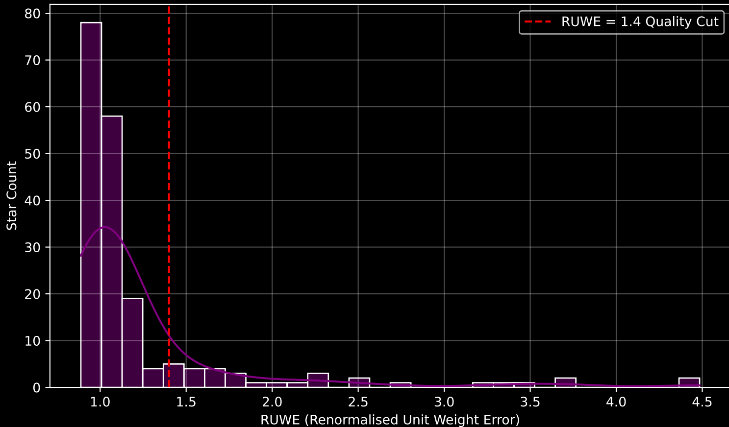
GALAH DR4 Field [8439] RUWE Distribution (n= 191)
