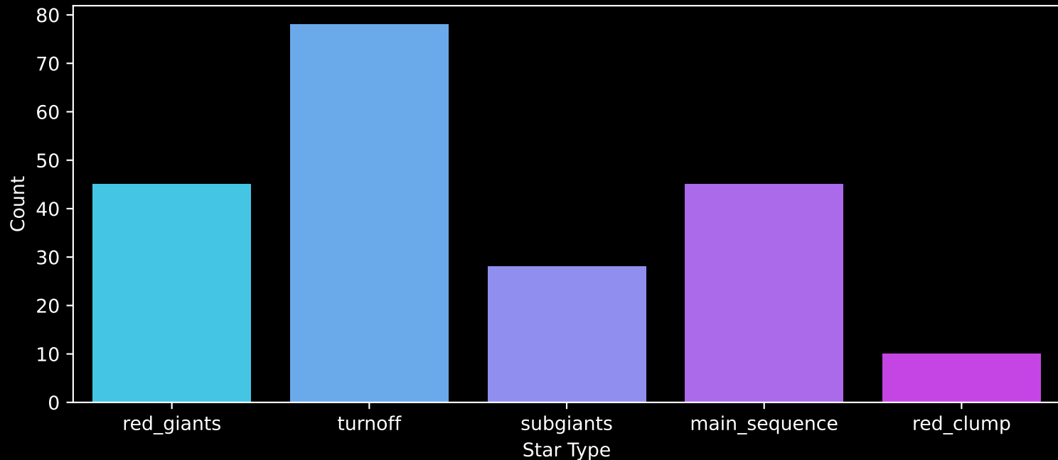
GALAH DR4 Field: [8439] Count plot of Star Type
